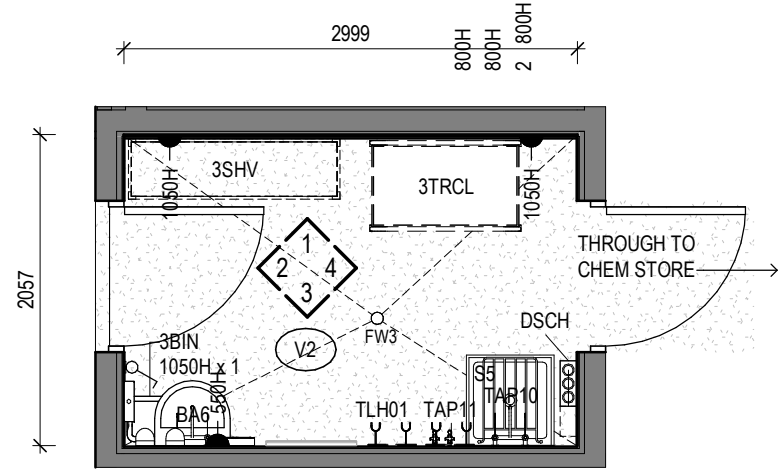
3 RACF-CLEANER - TYPE 2 Scale 1 : 50
