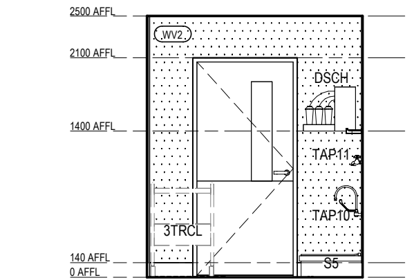
RACF BOH - CLEANER - TYPE 2 ELEVATION 4 Scale 1 : 50
