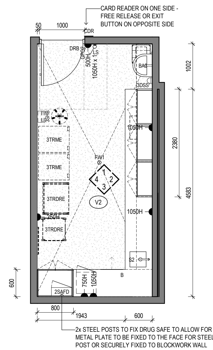
5 RACF-TREATMENT Scale 1 : 50
