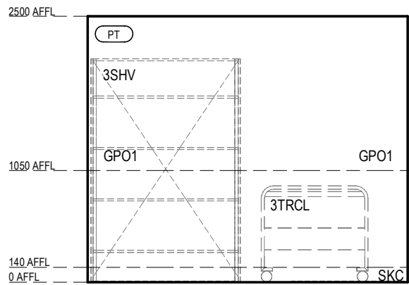
RACF BOH - CLEANER - TYPE 2 ELEVATION 1 Scale 1 : 50
