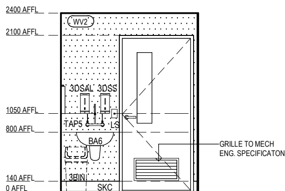
RACF BOH - CLEANER - TYPE 1 ELEVATION 1 Scale 1 : 50
