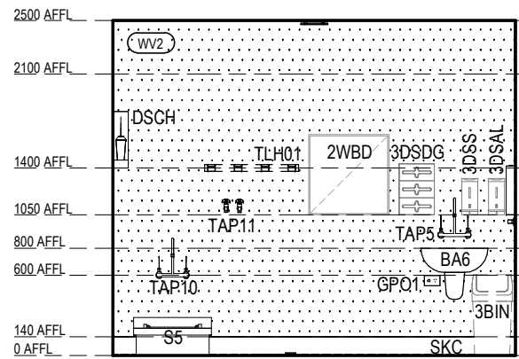
RACF BOH - CLEANER - TYPE 2 ELEVATION 3 Scale 1 : 50
