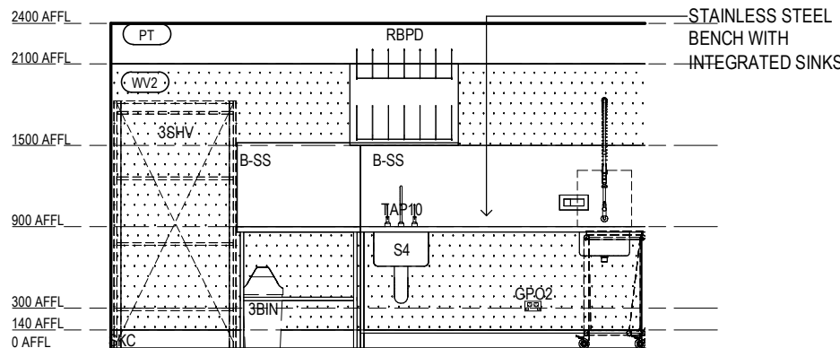
RACF BOH - SLUICE ELEVATION 1 Scale 1 : 50
