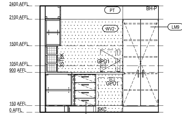
RACF BOH - TREATMENT ELEVATION 3 Scale 1 : 50
